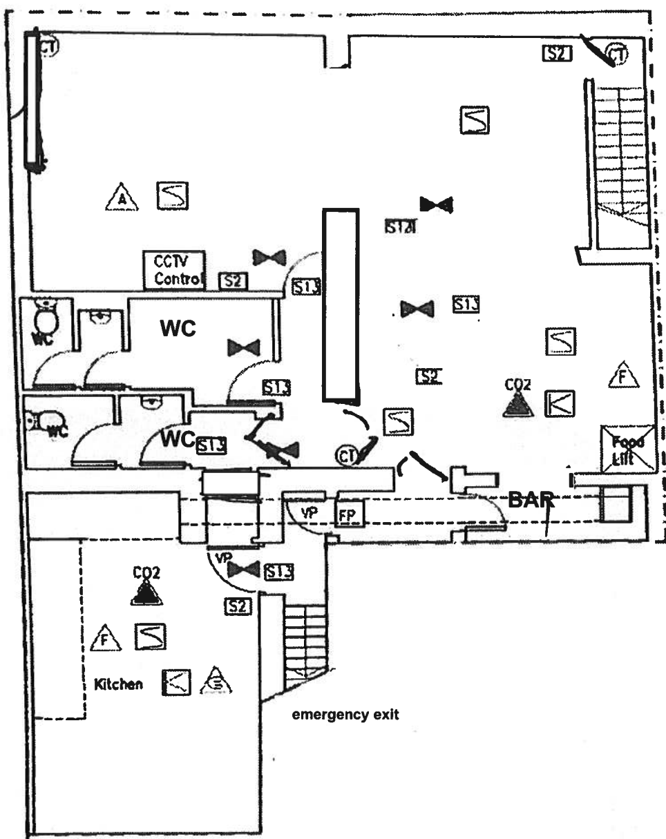
BASEMENT FLOOR PLAN 'Scale 1:100
